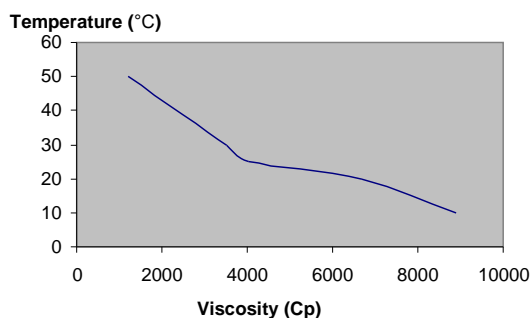
Viscosity variation with temperature
